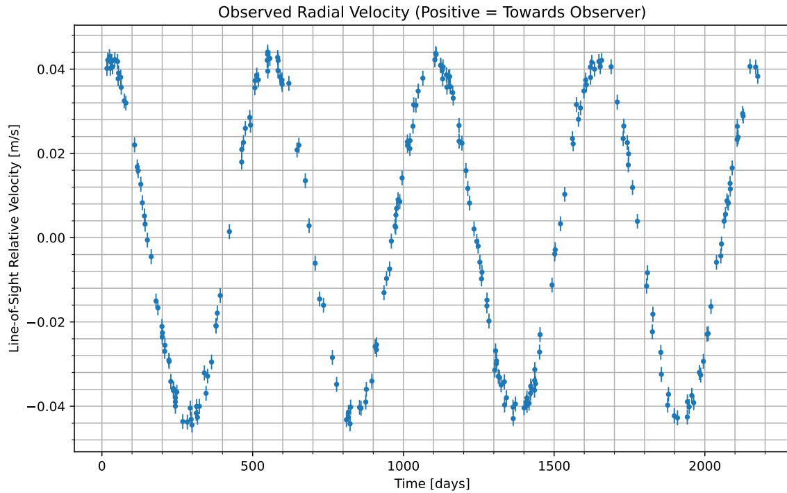
Figure 1: We have isolated the radial velocity of the host star due to the candidate planet. Data begins at UTC 2084-11-16/18:25. Positive values indicate the velocity at which the star is moving towards us; negative indicate the velocity at which it is moving away.
