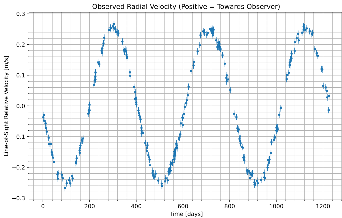
Figure 1: We have isolated the radial velocity of the host star due to the candidate planet. Data begins at UTC 2069-06-13/13:02. Positive values indicate the velocity at which the star is moving towards us; negative indicate the velocity at which it is moving away.
