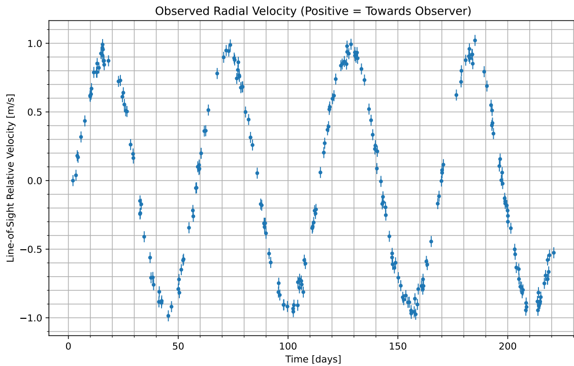
Figure 1: We have isolated the radial velocity of the host star due to the candidate planet. Data begins at UTC 2091-12-28/04:05. Positive values indicate the velocity at which the star is moving towards us; negative indicate the velocity at which it is moving away.
