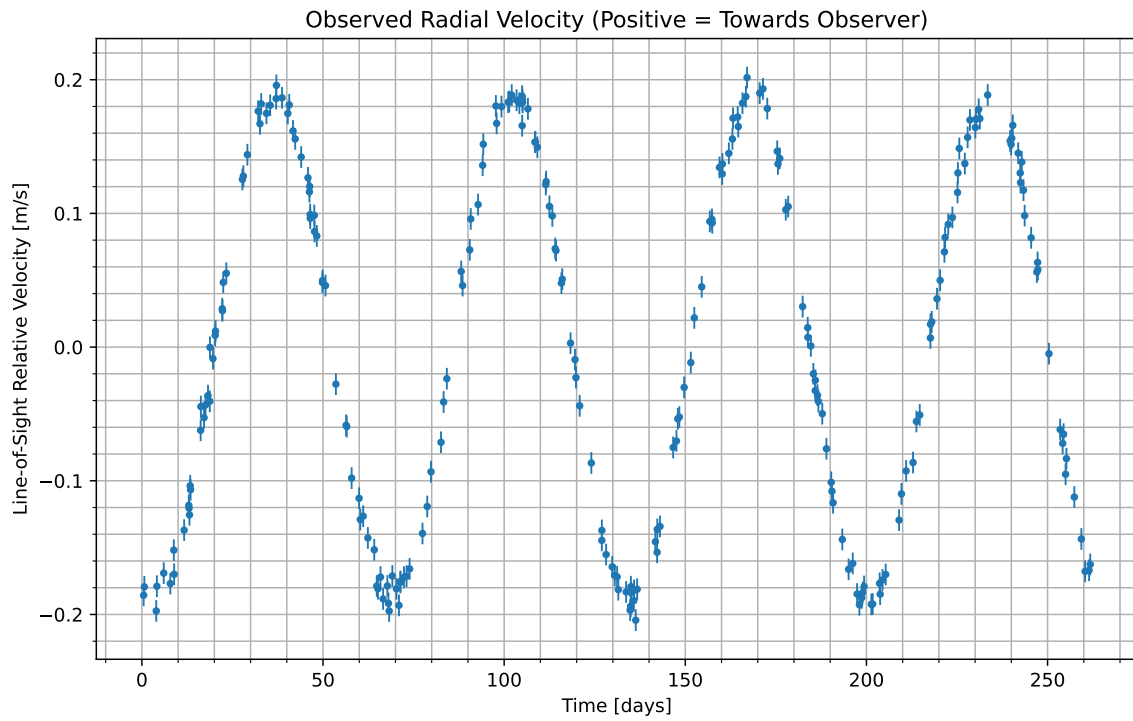
Figure 1: We have isolated the radial velocity of the host star due to the candidate planet. Data begins at UTC 2076-03-11/00:12. Positive values indicate the velocity at which the star is moving towards us; negative indicate the velocity at which it is moving away.
