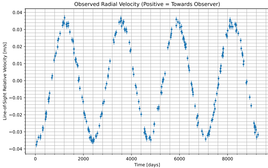
Figure 1: We have isolated the radial velocity of the host star due to the candidate planet. Data begins at UTC 2063-11-13/15:03. Positive values indicate the velocity at which the star is moving towards us; negative indicate the velocity at which it is moving away.
