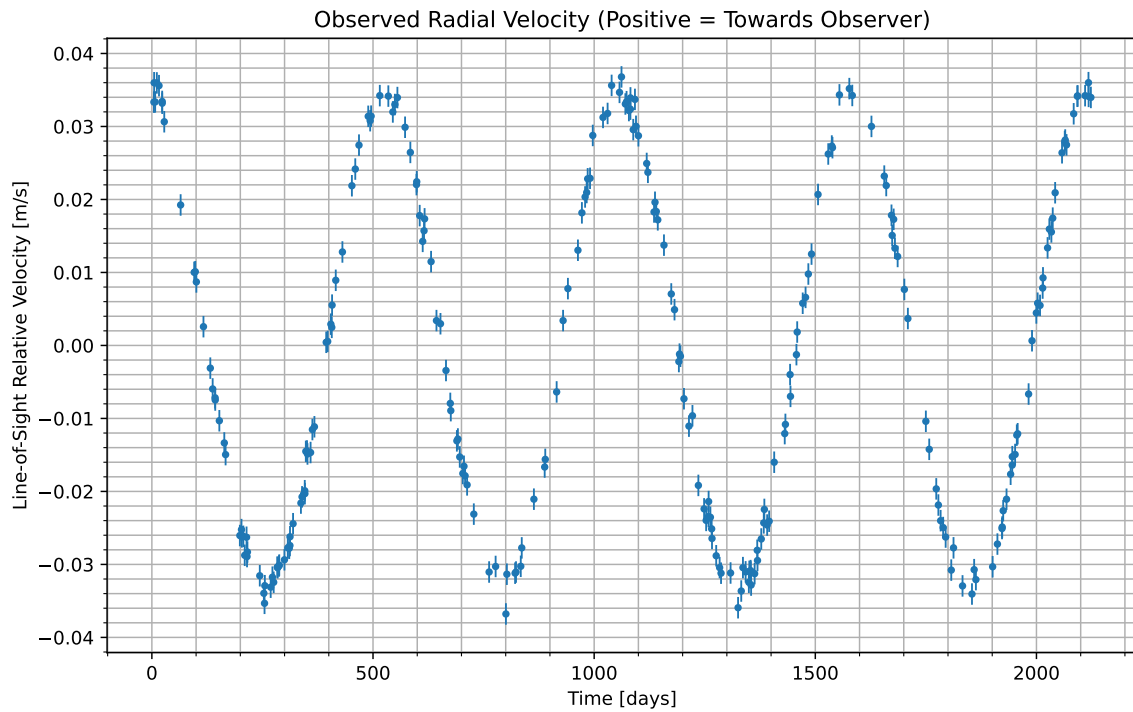
Figure 1: We have isolated the radial velocity of the host star due to the candidate planet. Data begins at UTC 2073-12-21/21:59. Positive values indicate the velocity at which the star is moving towards us; negative indicate the velocity at which it is moving away.
