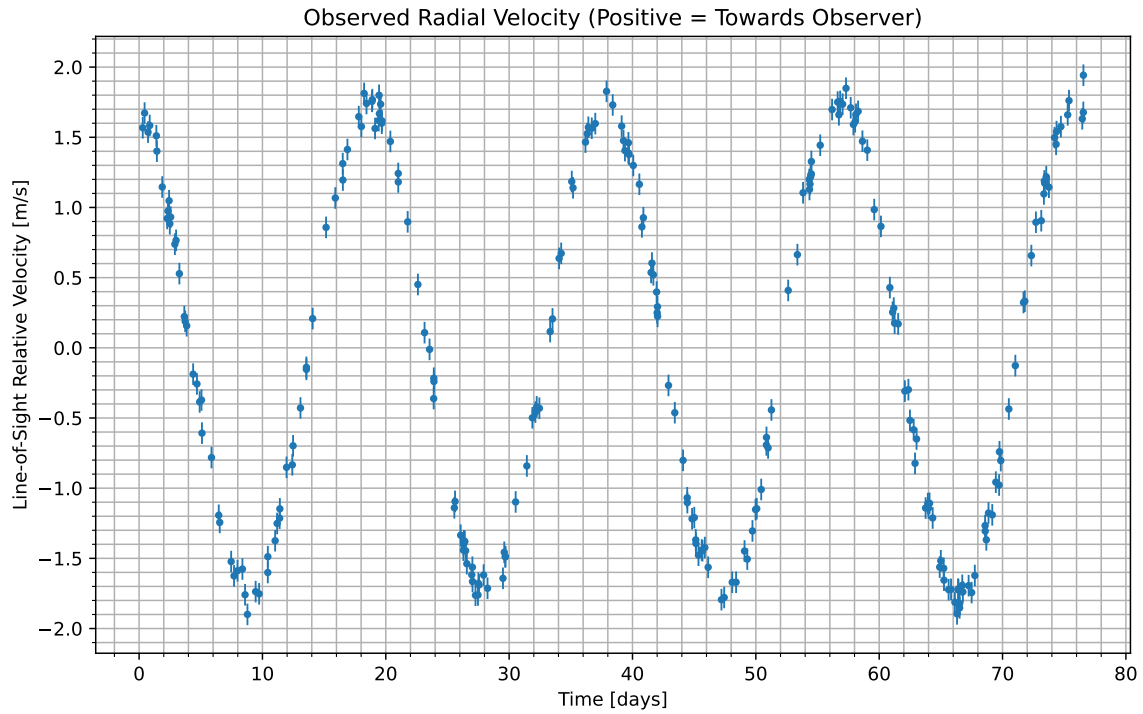
Figure 1: We have isolated the radial velocity of the host star due to the candidate planet. Data begins at UTC 2094-10-03/00:25. Positive values indicate the velocity at which the star is moving towards us; negative indicate the velocity at which it is moving away.
