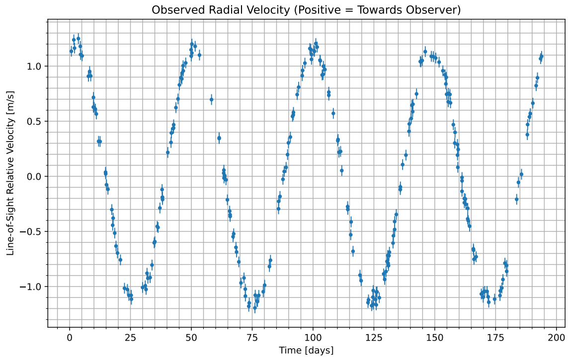
Figure 1: We have isolated the radial velocity of the host star due to the candidate planet. Data begins at UTC 2092-11-23/18:12. Positive values indicate the velocity at which the star is moving towards us; negative indicate the velocity at which it is moving away.
