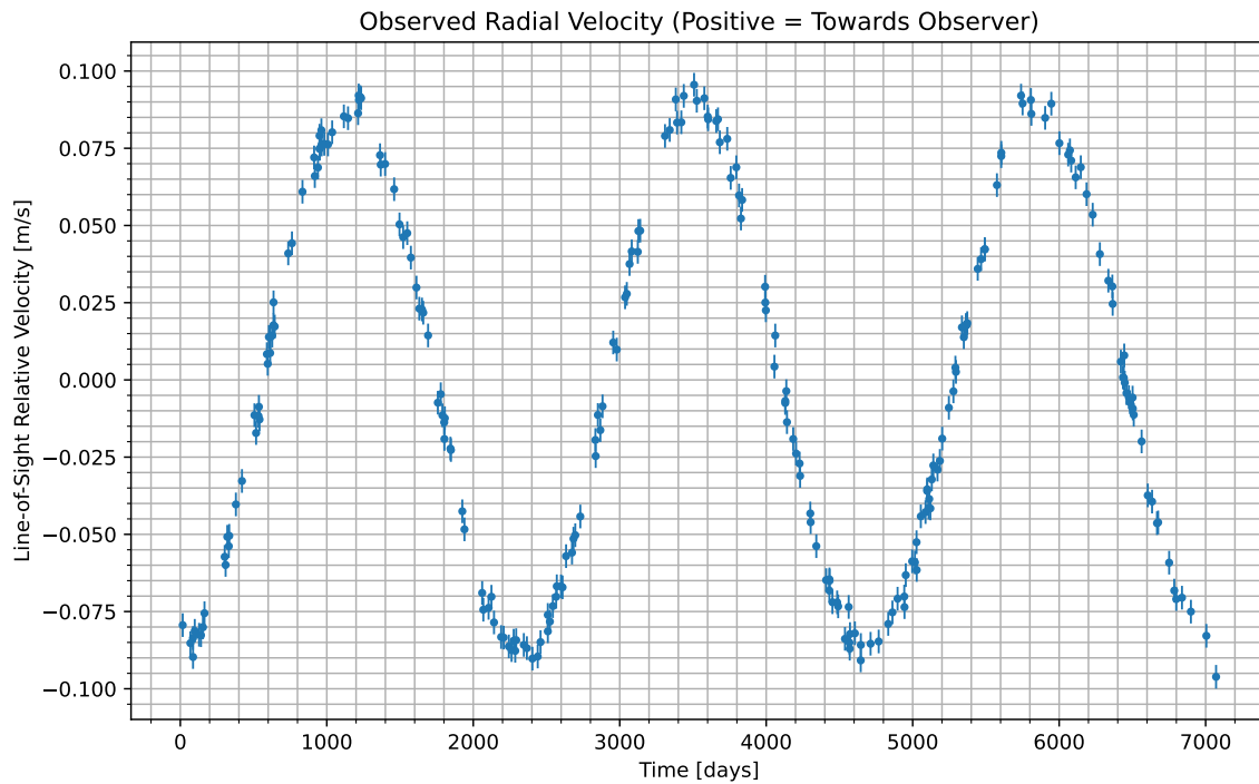
Figure 1: We have isolated the radial velocity of the host star due to the candidate planet. Data begins at UTC 2061-12-17/09:27. Positive values indicate the velocity at which the star is moving towards us; negative indicate the velocity at which it is moving away.
