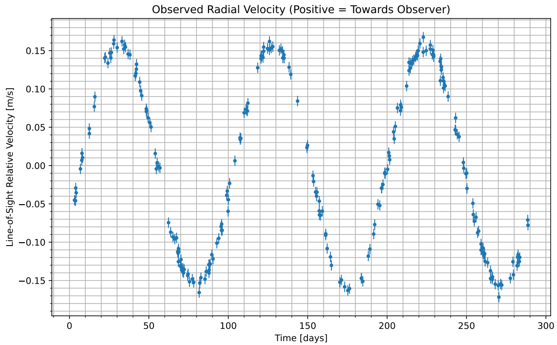
Figure 1: We have isolated the radial velocity of the host star due to the candidate planet. Data begins at UTC 2071-03-28/08:56. Positive values indicate the velocity at which the star is moving towards us; negative indicate the velocity at which it is moving away.
