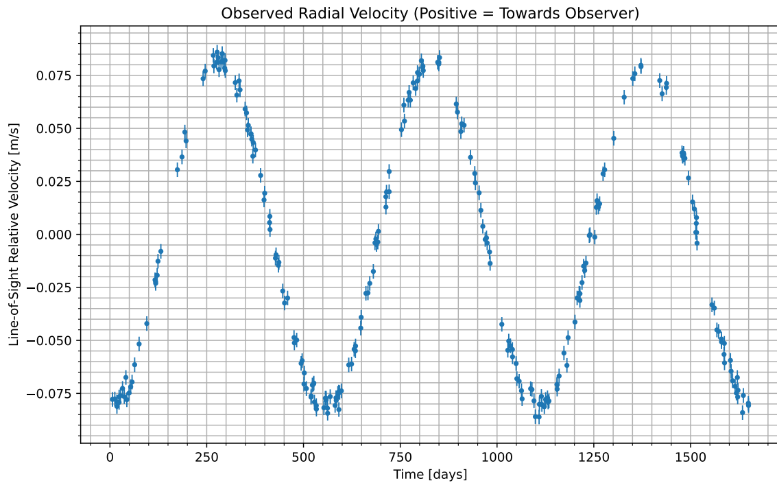
Figure 1: We have isolated the radial velocity of the host star due to the candidate planet. Data begins at UTC 2085-11-02/13:53. Positive values indicate the velocity at which the star is moving towards us; negative indicate the velocity at which it is moving away.
