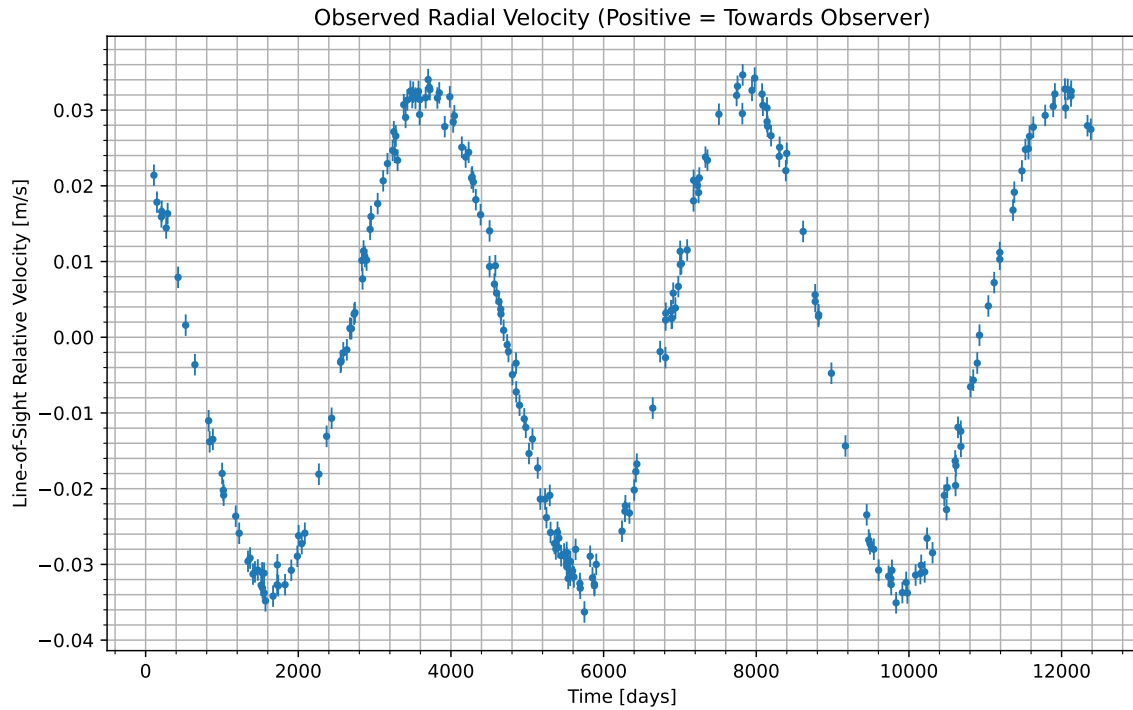
Figure 1: We have isolated the radial velocity of the host star due to the candidate planet. Data begins at UTC 2040-01-25/10:46. Positive values indicate the velocity at which the star is moving towards us; negative indicate the velocity at which it is moving away.
