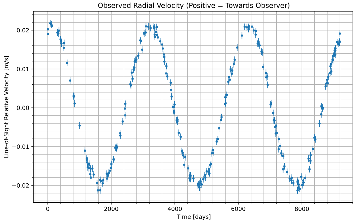
Figure 1: We have isolated the radial velocity of the host star due to the candidate planet. Data begins at UTC 2056-04-08/10:30. Positive values indicate the velocity at which the star is moving towards us; negative indicate the velocity at which it is moving away.
