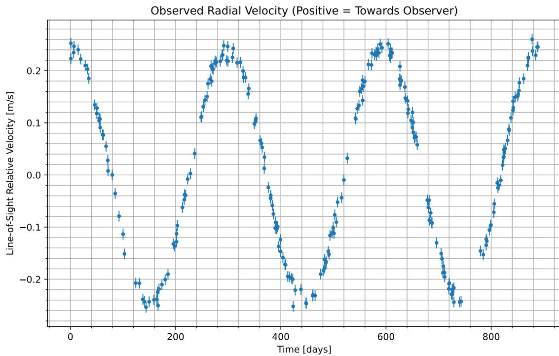
Figure 1: We have isolated the radial velocity of the host star due to the candidate planet. Data begins at UTC 2089-04-21/08:13. Positive values indicate the velocity at which the star is moving towards us; negative indicate the velocity at which it is moving away.
