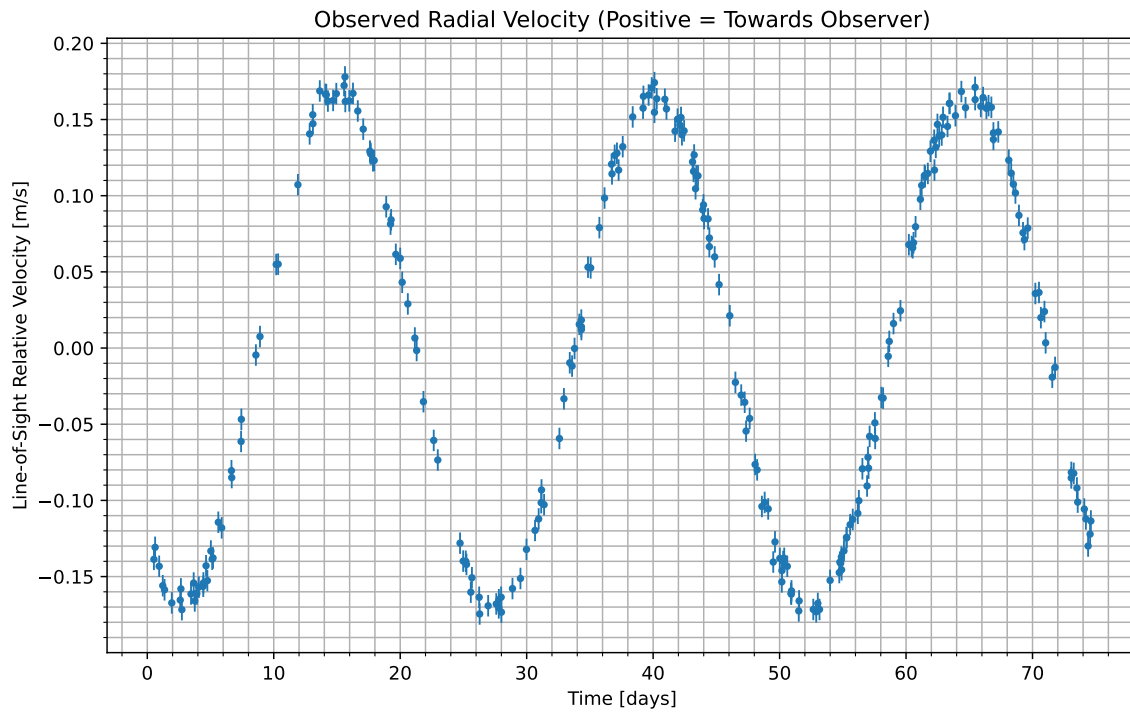
Figure 1: We have isolated the radial velocity of the host star due to the candidate planet. Data begins at UTC 2095-06-17/12:32. Positive values indicate the velocity at which the star is moving towards us; negative indicate the velocity at which it is moving away.
