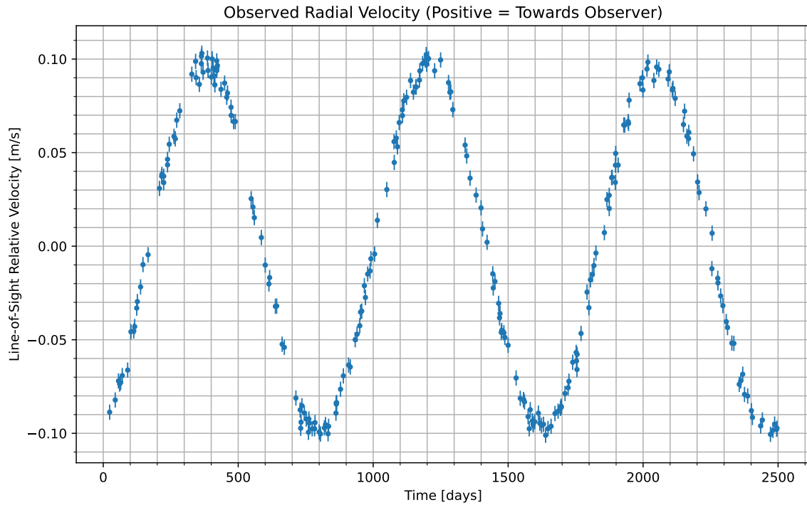
Figure 1: We have isolated the radial velocity of the host star due to the candidate planet. Data begins at UTC 2090-03-14/22:40. Positive values indicate the velocity at which the star is moving towards us; negative indicate the velocity at which it is moving away.
