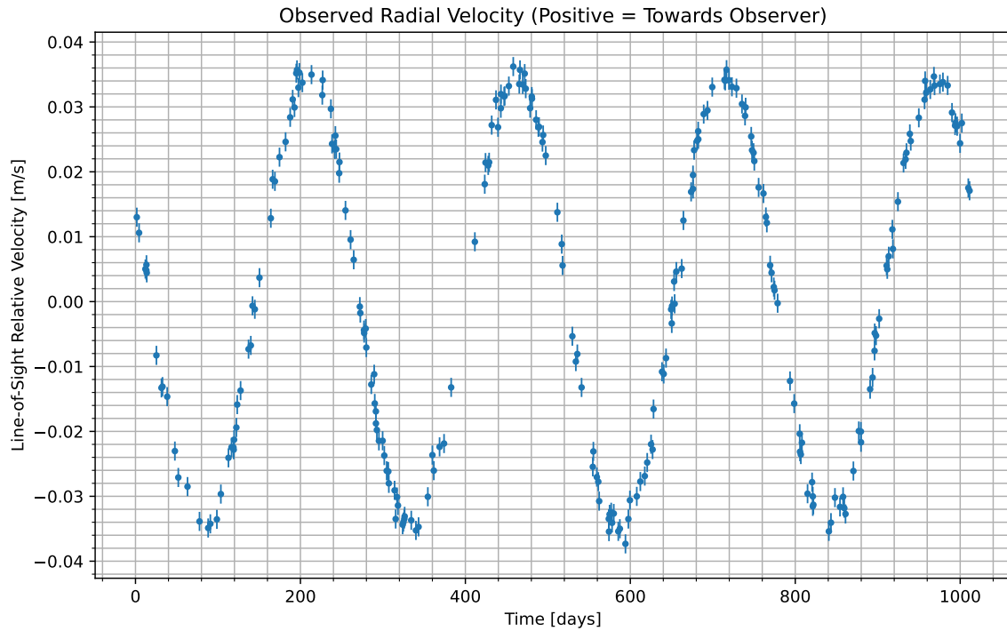
Figure 1: We have isolated the radial velocity of the host star due to the candidate planet. Data begins at UTC 2083-04-15/23:43. Positive values indicate the velocity at which the star is moving towards us; negative indicate the velocity at which it is moving away.
