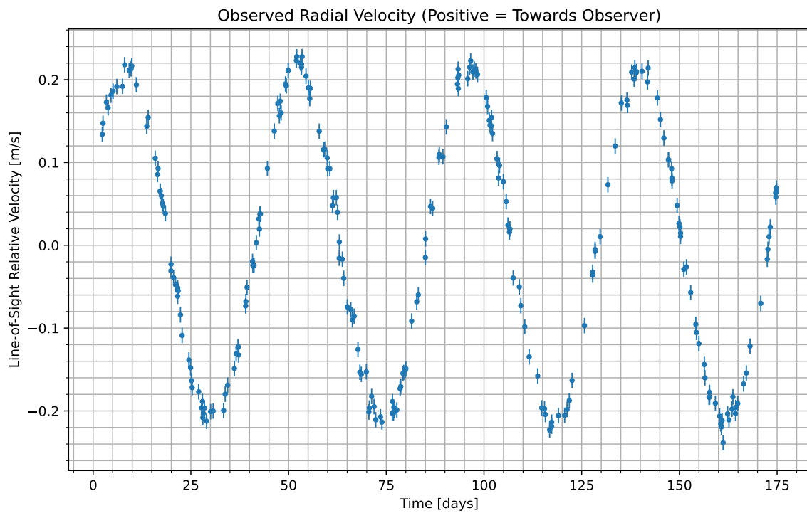
Figure 1: We have isolated the radial velocity of the host star due to the candidate planet. Data begins at UTC 2090-02-26/14:51. Positive values indicate the velocity at which the star is moving towards us; negative indicate the velocity at which it is moving away.
