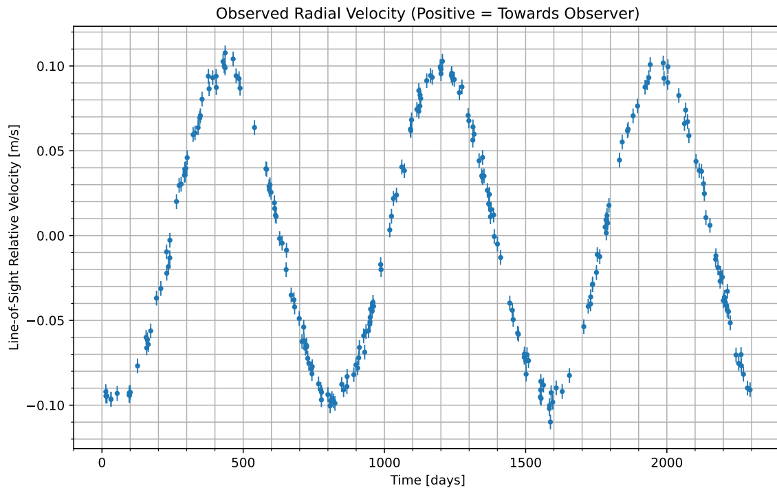
Figure 1: We have isolated the radial velocity of the host star due to the candidate planet. Data begins at UTC 2089-09-06/00:32. Positive values indicate the velocity at which the star is moving towards us; negative indicate the velocity at which it is moving away.
