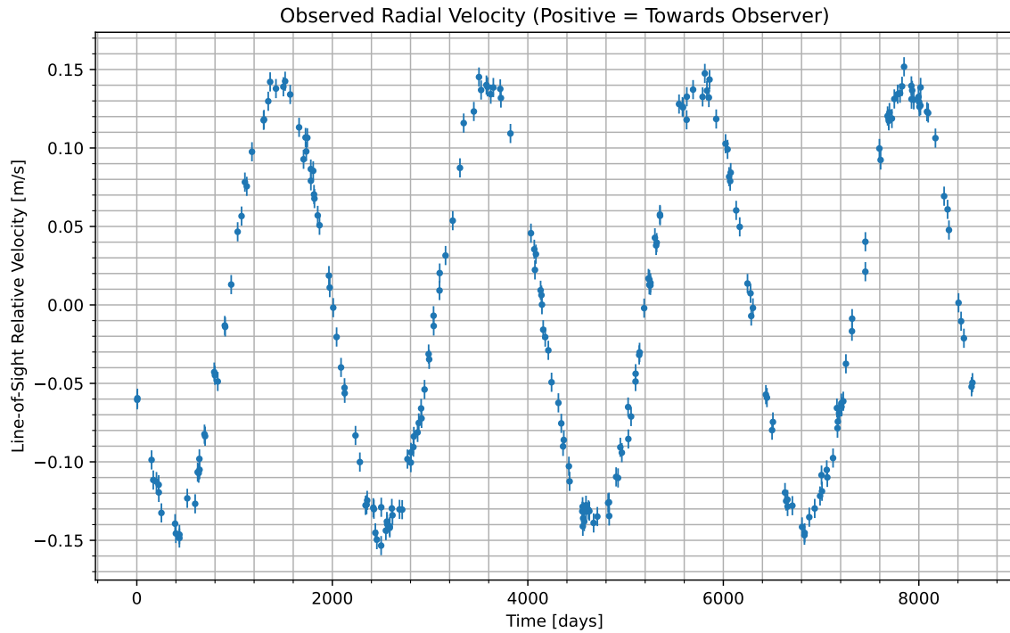
Figure 1: We have isolated the radial velocity of the host star due to the candidate planet. Data begins at UTC 2054-09-24/18:22. Positive values indicate the velocity at which the star is moving towards us; negative indicate the velocity at which it is moving away.
