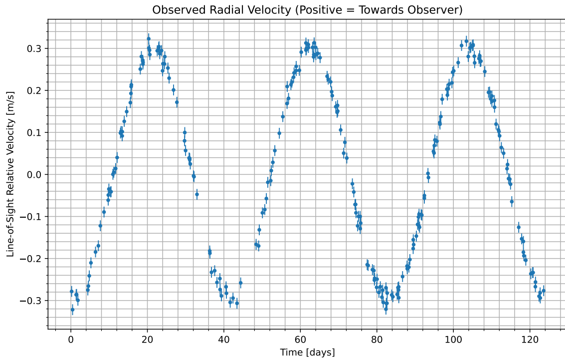
Figure 1: We have isolated the radial velocity of the host star due to the candidate planet. Data begins at UTC 2099-08-21/18:13. Positive values indicate the velocity at which the star is moving towards us; negative indicate the velocity at which it is moving away.
