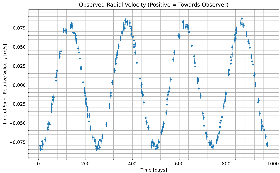
Figure 1: We have isolated the radial velocity of the host star due to the candidate planet. Data begins at UTC 2076-08-08/14:40. Positive values indicate the velocity at which the star is moving towards us; negative indicate the velocity at which it is moving away.
