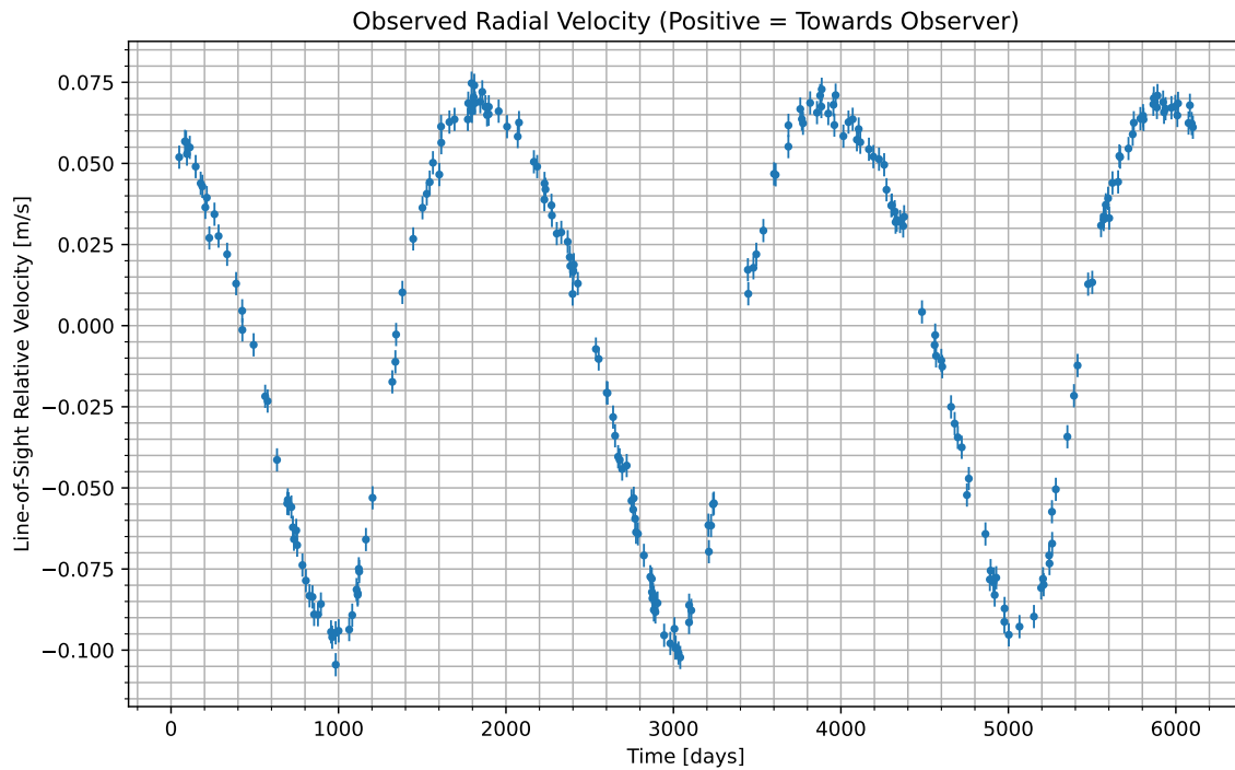
Figure 1: We have isolated the radial velocity of the host star due to the candidate planet. Data begins at UTC 2058-09-08/16:08. Positive values indicate the velocity at which the star is moving towards us; negative indicate the velocity at which it is moving away.
