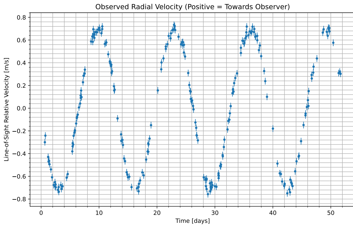
Figure 1: We have isolated the radial velocity of the host star due to the candidate planet. Data begins at UTC 2088-10-21/23:45. Positive values indicate the velocity at which the star is moving towards us; negative indicate the velocity at which it is moving away.
