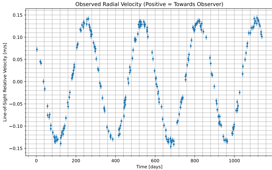
Figure 1: We have isolated the radial velocity of the host star due to the candidate planet. Data begins at UTC 2083-01-04/18:38. Positive values indicate the velocity at which the star is moving towards us; negative indicate the velocity at which it is moving away.
