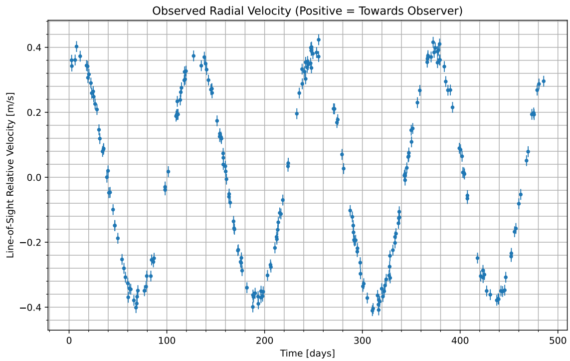
Figure 1: We have isolated the radial velocity of the host star due to the candidate planet. Data begins at UTC 2093-06-06/05:12. Positive values indicate the velocity at which the star is moving towards us; negative indicate the velocity at which it is moving away.
