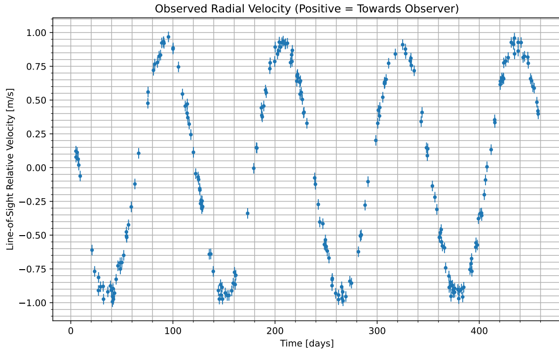
Figure 1: We have isolated the radial velocity of the host star due to the candidate planet. Data begins at UTC 2073-03-28/13:22. Positive values indicate the velocity at which the star is moving towards us; negative indicate the velocity at which it is moving away.
