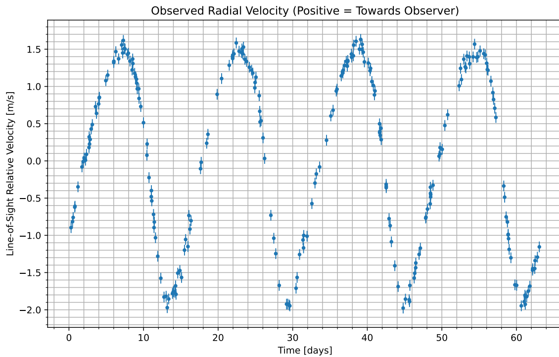
Figure 1: We have isolated the radial velocity of the host star due to the candidate planet. Data begins at UTC 2093-03-10/21:23. Positive values indicate the velocity at which the star is moving towards us; negative indicate the velocity at which it is moving away.
