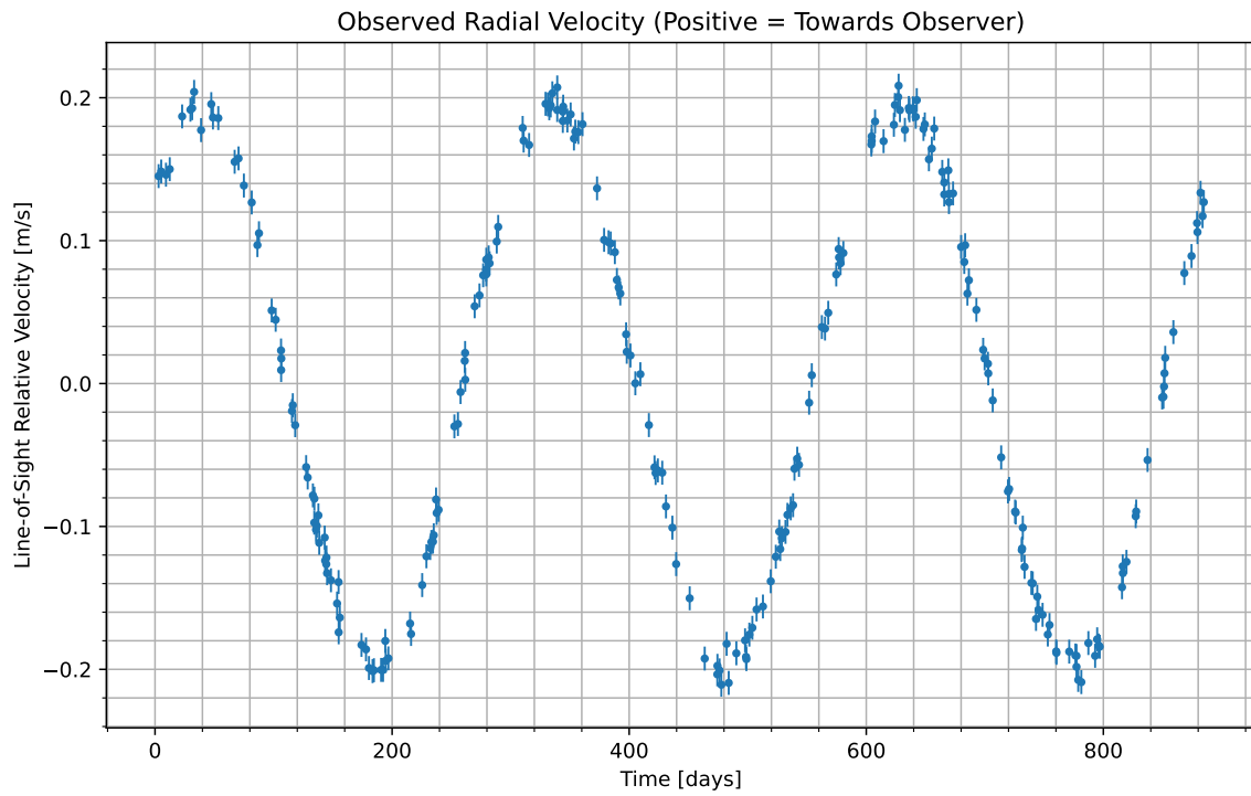
Figure 1: We have isolated the radial velocity of the host star due to the candidate planet. Data begins at UTC 2093-06-30/17:01. Positive values indicate the velocity at which the star is moving towards us; negative indicate the velocity at which it is moving away.
