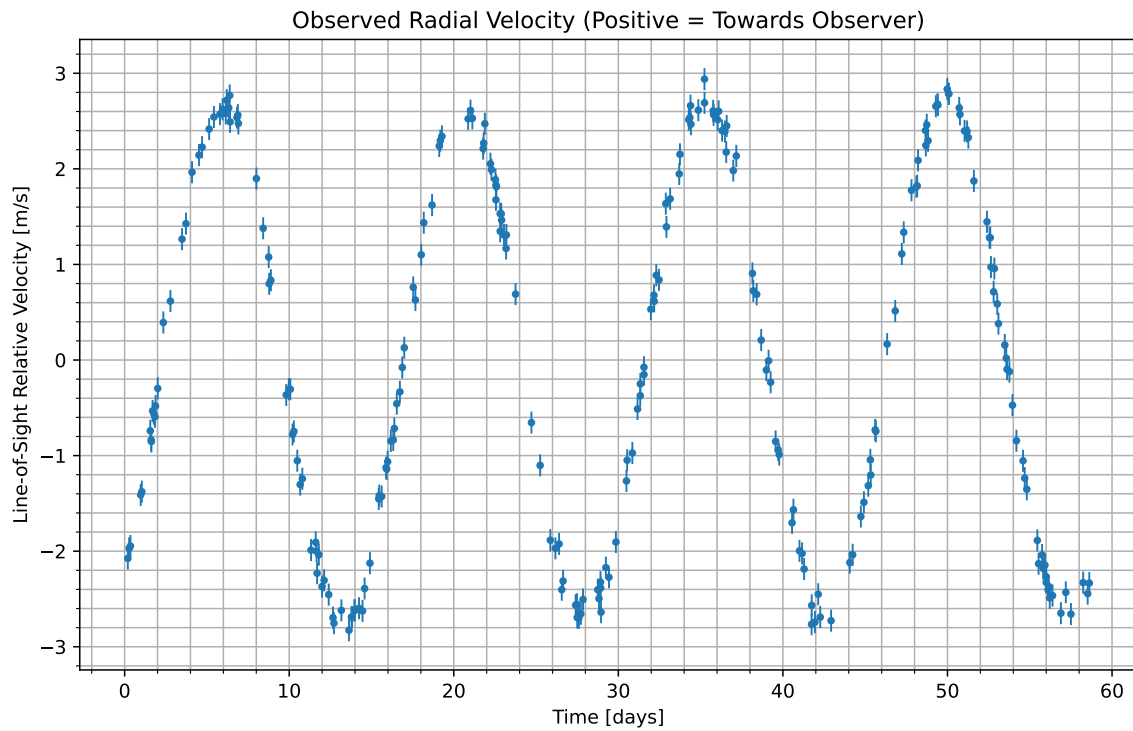
Figure 1: We have isolated the radial velocity of the host star due to the candidate planet. Data begins at UTC 2093-02-02/17:26. Positive values indicate the velocity at which the star is moving towards us; negative indicate the velocity at which it is moving away.
