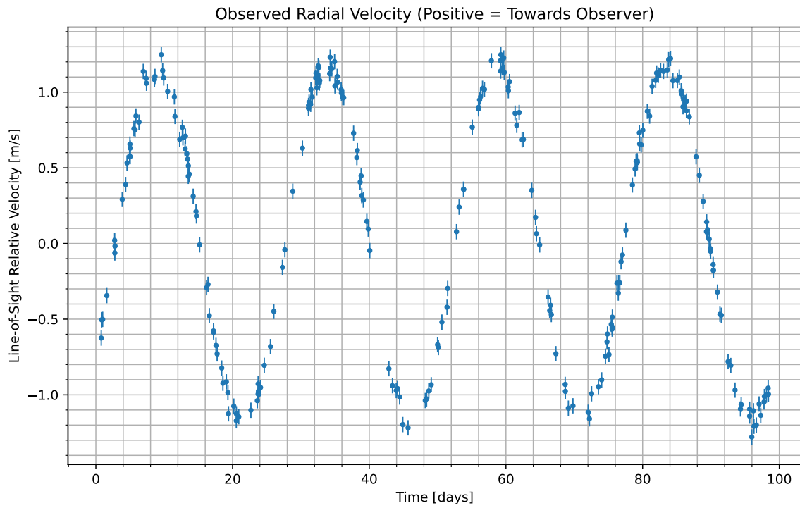
Figure 1: We have isolated the radial velocity of the host star due to the candidate planet. Data begins at UTC 2084-01-19/08:36. Positive values indicate the velocity at which the star is moving towards us; negative indicate the velocity at which it is moving away.
