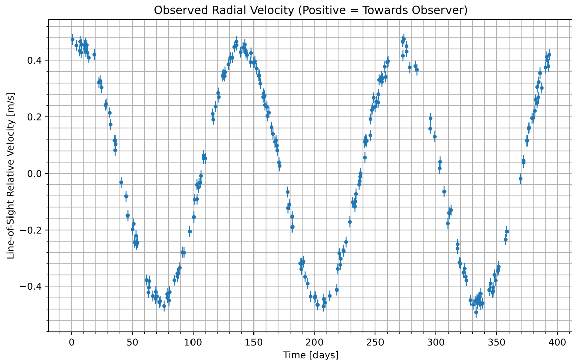
Figure 1: We have isolated the radial velocity of the host star due to the candidate planet. Data begins at UTC 2082-01-04/05:11. Positive values indicate the velocity at which the star is moving towards us; negative indicate the velocity at which it is moving away.
