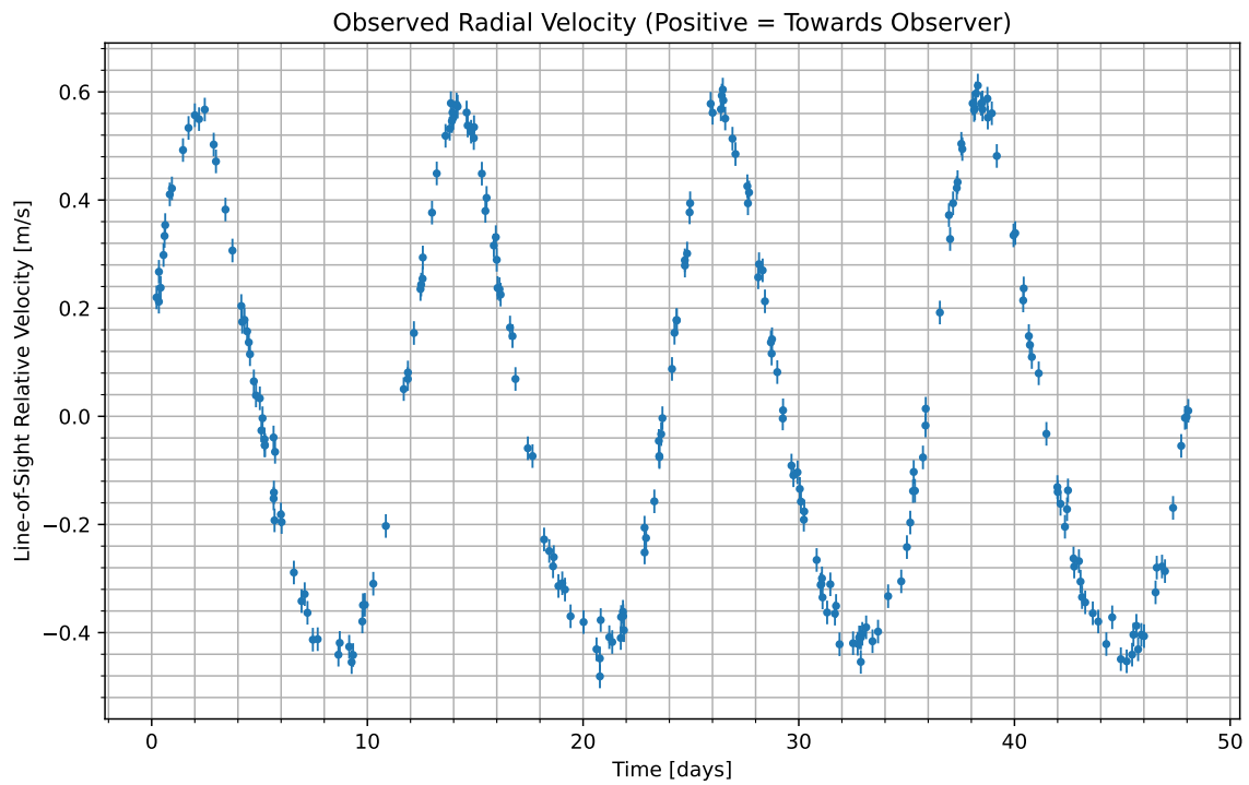
Figure 1: We have isolated the radial velocity of the host star due to the candidate planet. Data begins at UTC 2100-08-08/13:22. Positive values indicate the velocity at which the star is moving towards us; negative indicate the velocity at which it is moving away.
