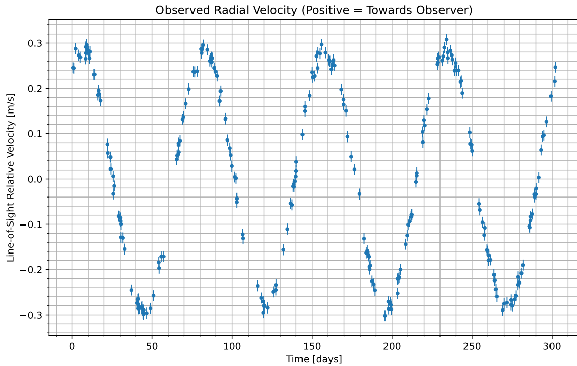
Figure 1: We have isolated the radial velocity of the host star due to the candidate planet. Data begins at UTC 2080-05-29/03:37. Positive values indicate the velocity at which the star is moving towards us; negative indicate the velocity at which it is moving away.
