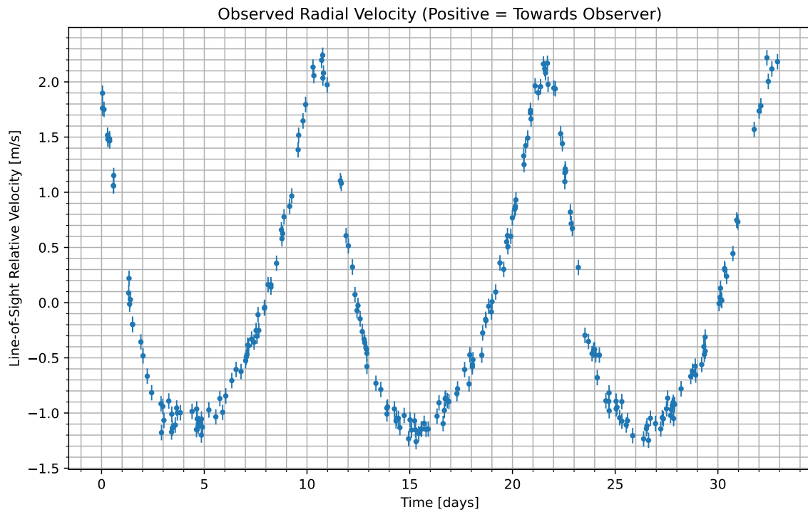
Figure 1: We have isolated the radial velocity of the host star due to the candidate planet. Data begins at UTC 2097-05-07/07:57. Positive values indicate the velocity at which the star is moving towards us; negative indicate the velocity at which it is moving away.
