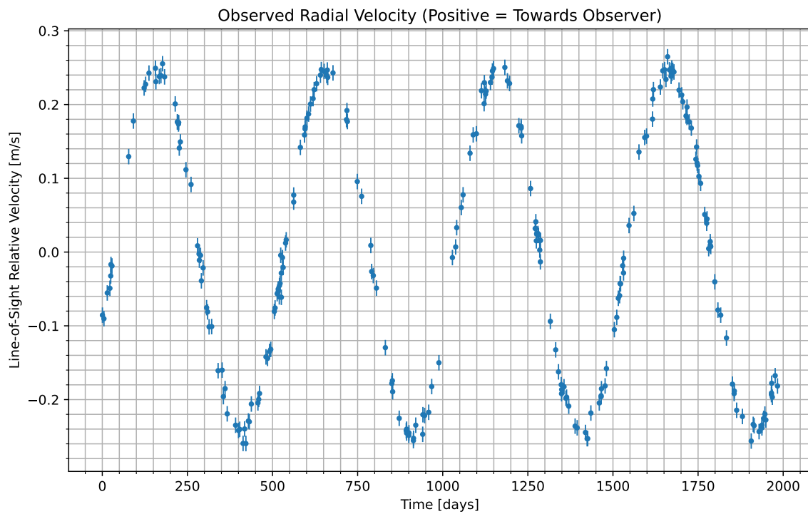
Figure 1: We have isolated the radial velocity of the host star due to the candidate planet. Data begins at UTC 2089-10-31/05:06. Positive values indicate the velocity at which the star is moving towards us; negative indicate the velocity at which it is moving away.
