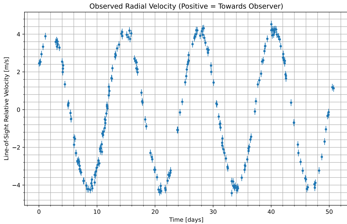
Figure 1: We have isolated the radial velocity of the host star due to the candidate planet. Data begins at UTC 2093-02-14/10:30. Positive values indicate the velocity at which the star is moving towards us; negative indicate the velocity at which it is moving away.
