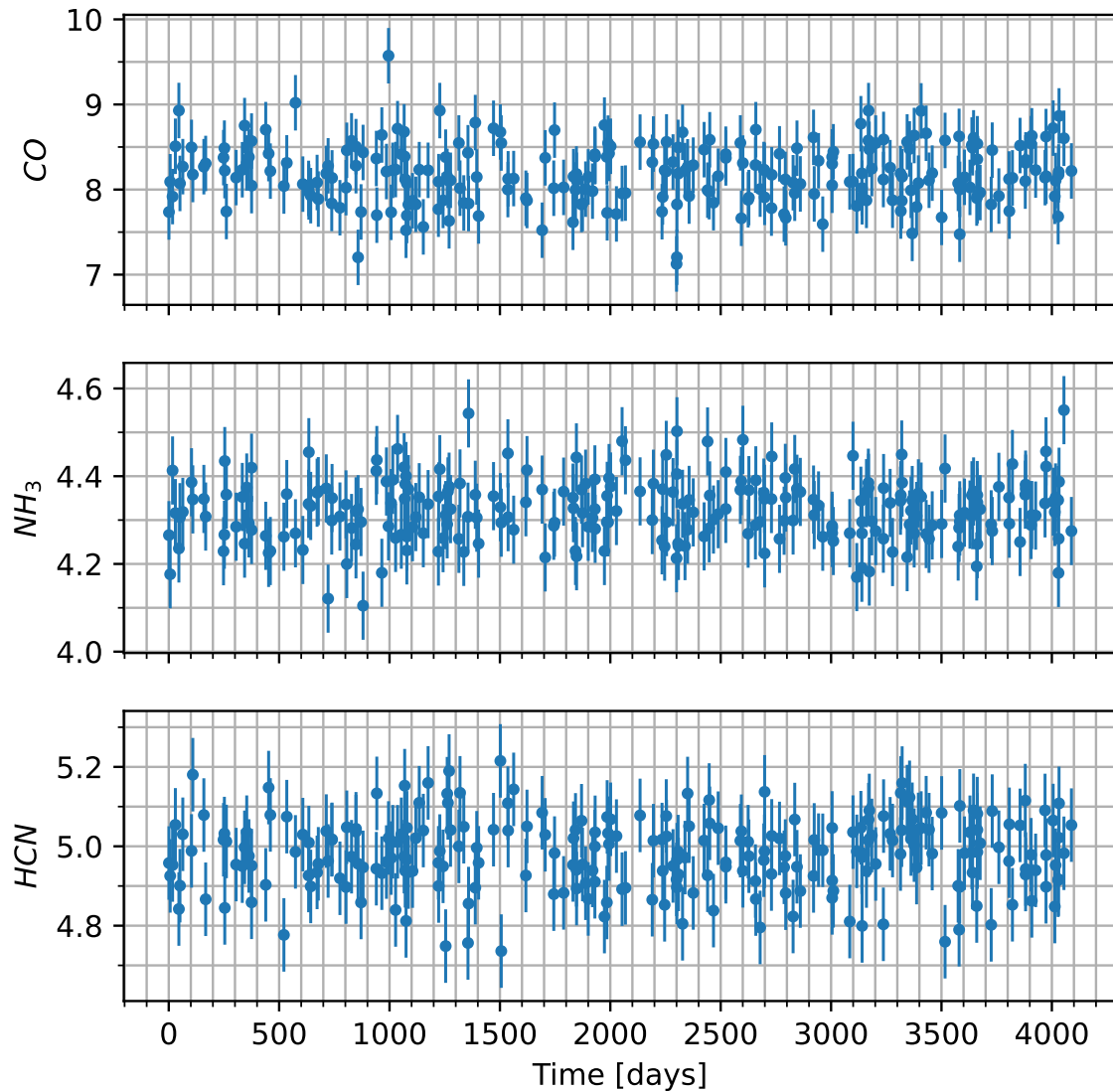
Figure 3: Concentration of various additional gases in the atmosphere of the candidate planet versus time. Note that the y-axis will usually only show the variation multiplied by some factor, shown in the upper left, and then added to some normal amount, also in the upper-left.
