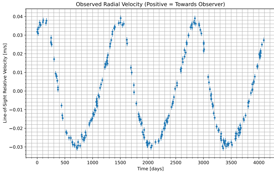
Figure 1: We have isolated the radial velocity of the host star due to the candidate planet. Data begins at UTC 2064-02-04/23:31. Positive values indicate the velocity at which the star is moving towards us; negative indicate the velocity at which it is moving away.
