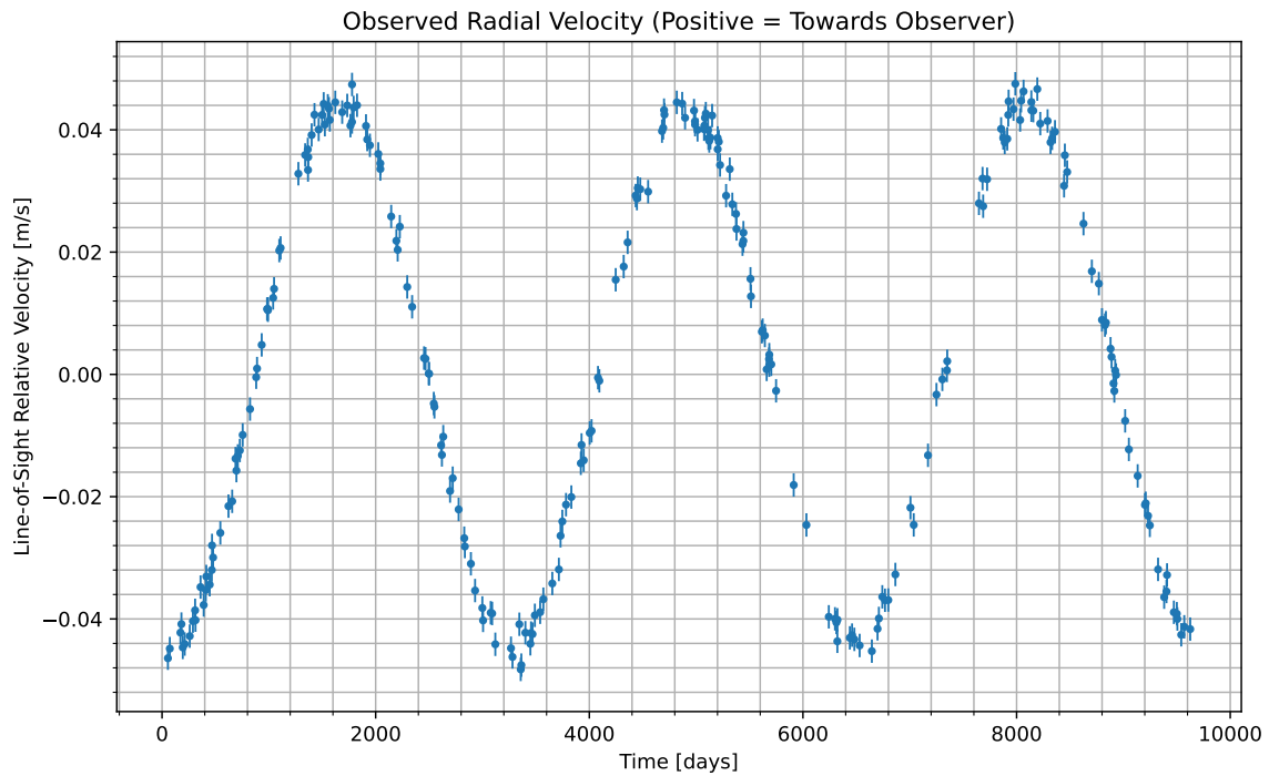
Figure 1: We have isolated the radial velocity of the host star due to the candidate planet. Data begins at UTC 2045-02-09/08:12. Positive values indicate the velocity at which the star is moving towards us; negative indicate the velocity at which it is moving away.
