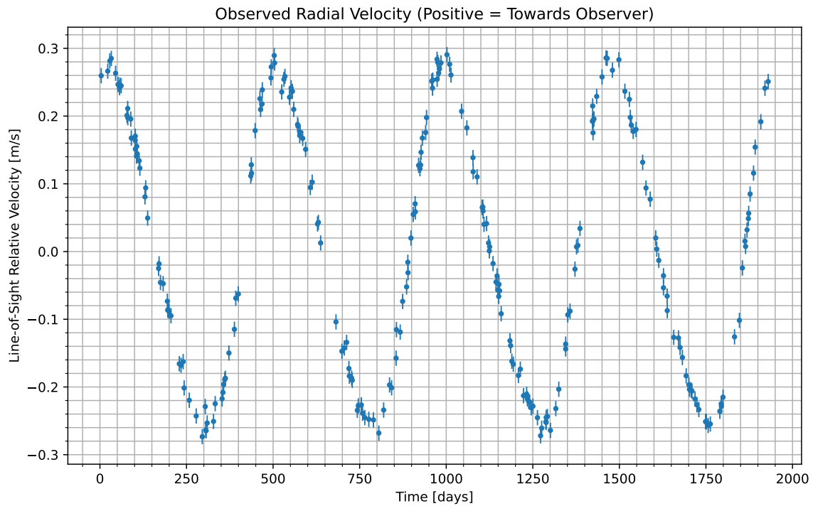
Figure 1: We have isolated the radial velocity of the host star due to the candidate planet. Data begins at UTC 2081-01-23/18:33. Positive values indicate the velocity at which the star is moving towards us; negative indicate the velocity at which it is moving away.
