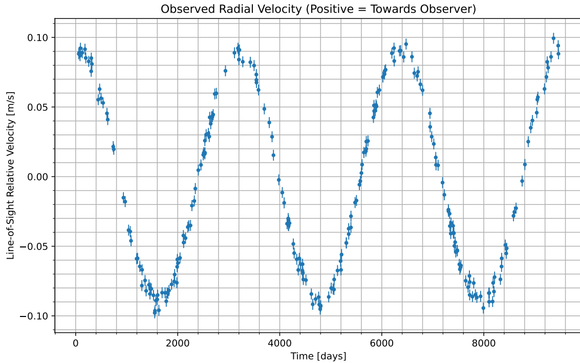
Figure 1: We have isolated the radial velocity of the host star due to the candidate planet. Data begins at UTC 2048-06-17/11:08. Positive values indicate the velocity at which the star is moving towards us; negative indicate the velocity at which it is moving away.
