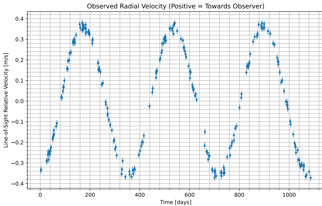
Figure 1: We have isolated the radial velocity of the host star due to the candidate planet. Data begins at UTC 2095-05-05/11:33. Positive values indicate the velocity at which the star is moving towards us; negative indicate the velocity at which it is moving away.
