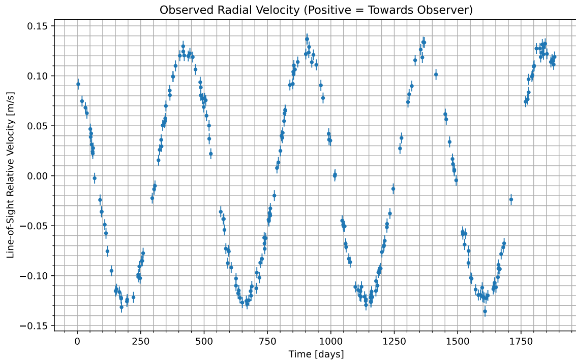
Figure 1: We have isolated the radial velocity of the host star due to the candidate planet. Data begins at UTC 2089-08-17/06:53. Positive values indicate the velocity at which the star is moving towards us; negative indicate the velocity at which it is moving away.
