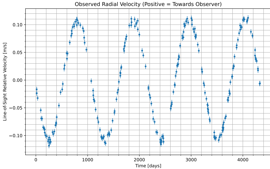
Figure 1: We have isolated the radial velocity of the host star due to the candidate planet. Data begins at UTC 2088-02-28/19:18. Positive values indicate the velocity at which the star is moving towards us; negative indicate the velocity at which it is moving away.
