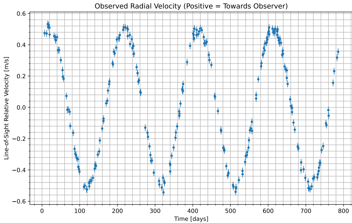
Figure 1: We have isolated the radial velocity of the host star due to the candidate planet. Data begins at UTC 2072-05-27/19:26. Positive values indicate the velocity at which the star is moving towards us; negative indicate the velocity at which it is moving away.
