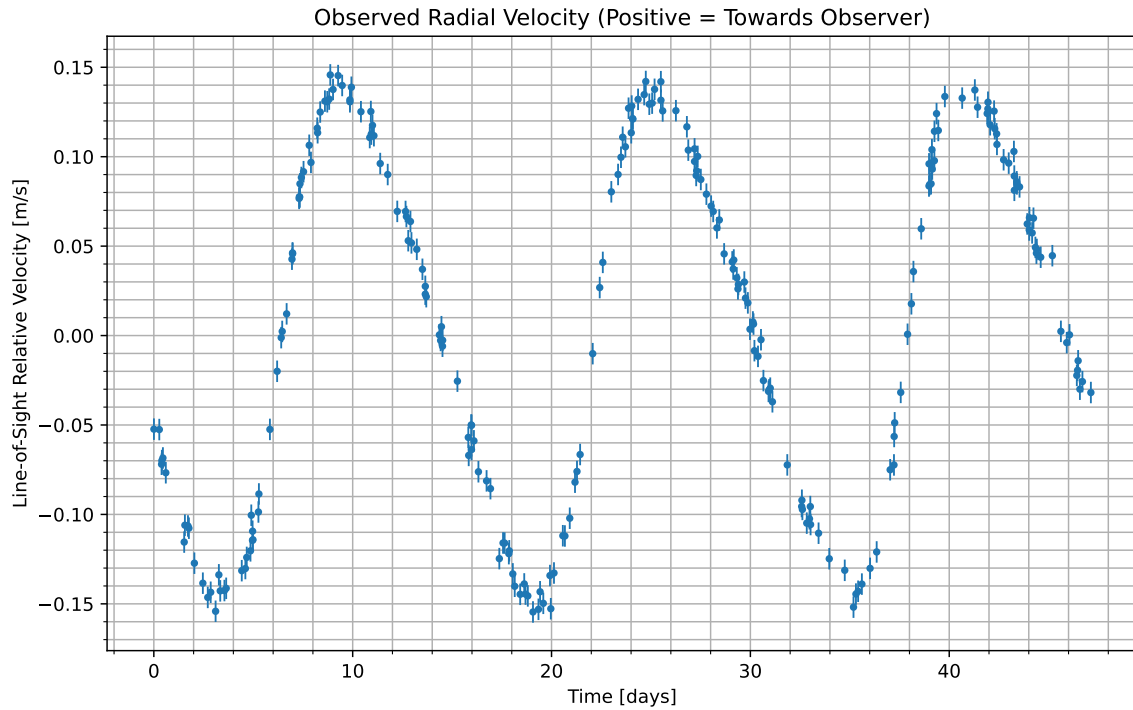
Figure 1: We have isolated the radial velocity of the host star due to the candidate planet. Data begins at UTC 2084-08-26/12:34. Positive values indicate the velocity at which the star is moving towards us; negative indicate the velocity at which it is moving away.
