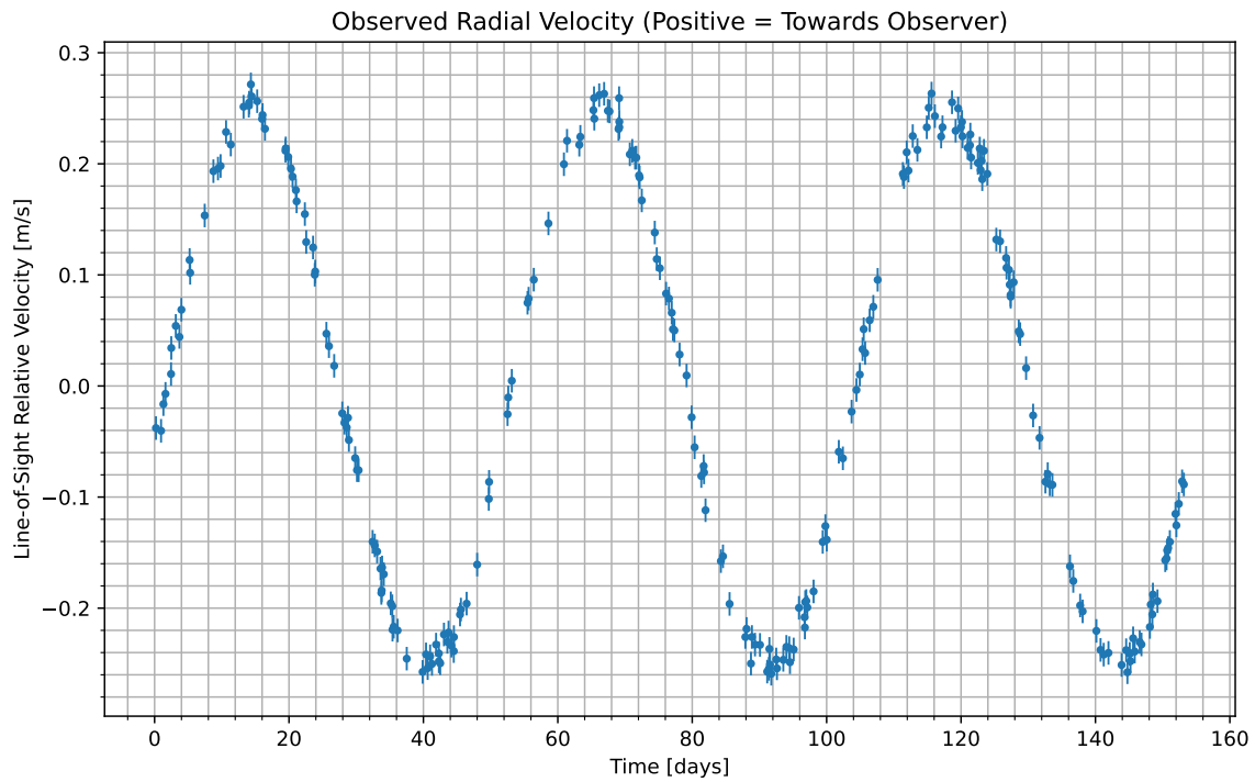
Figure 1: We have isolated the radial velocity of the host star due to the candidate planet. Data begins at UTC 2099-02-02/06:42. Positive values indicate the velocity at which the star is moving towards us; negative indicate the velocity at which it is moving away.
