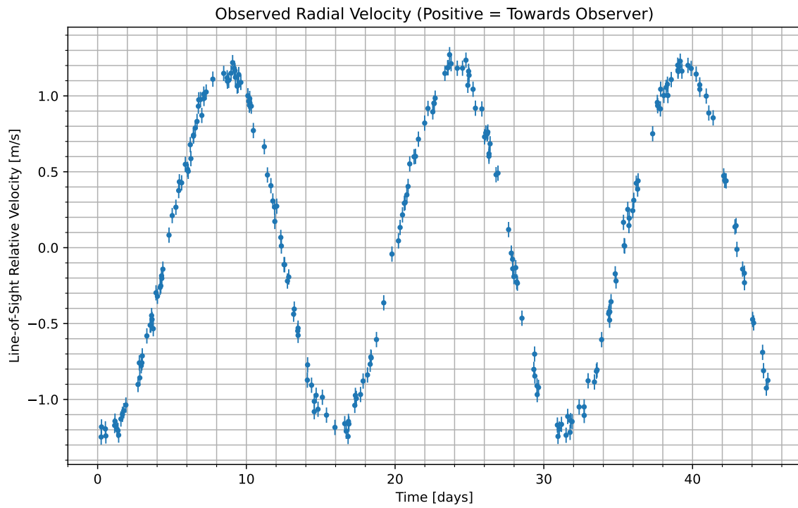
Figure 1: We have isolated the radial velocity of the host star due to the candidate planet. Data begins at UTC 2074-05-19/23:56. Positive values indicate the velocity at which the star is moving towards us; negative indicate the velocity at which it is moving away.
