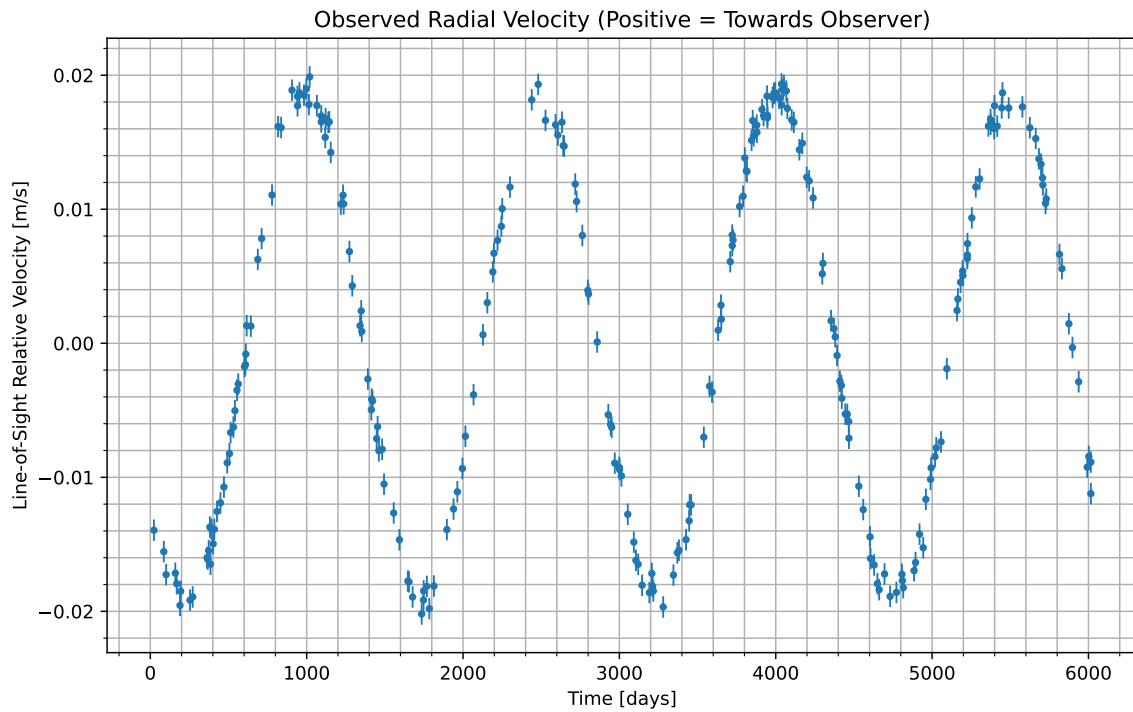
Figure 1: We have isolated the radial velocity of the host star due to the candidate planet. Data begins at UTC 2067-06-08/03:26. Positive values indicate the velocity at which the star is moving towards us; negative indicate the velocity at which it is moving away.
