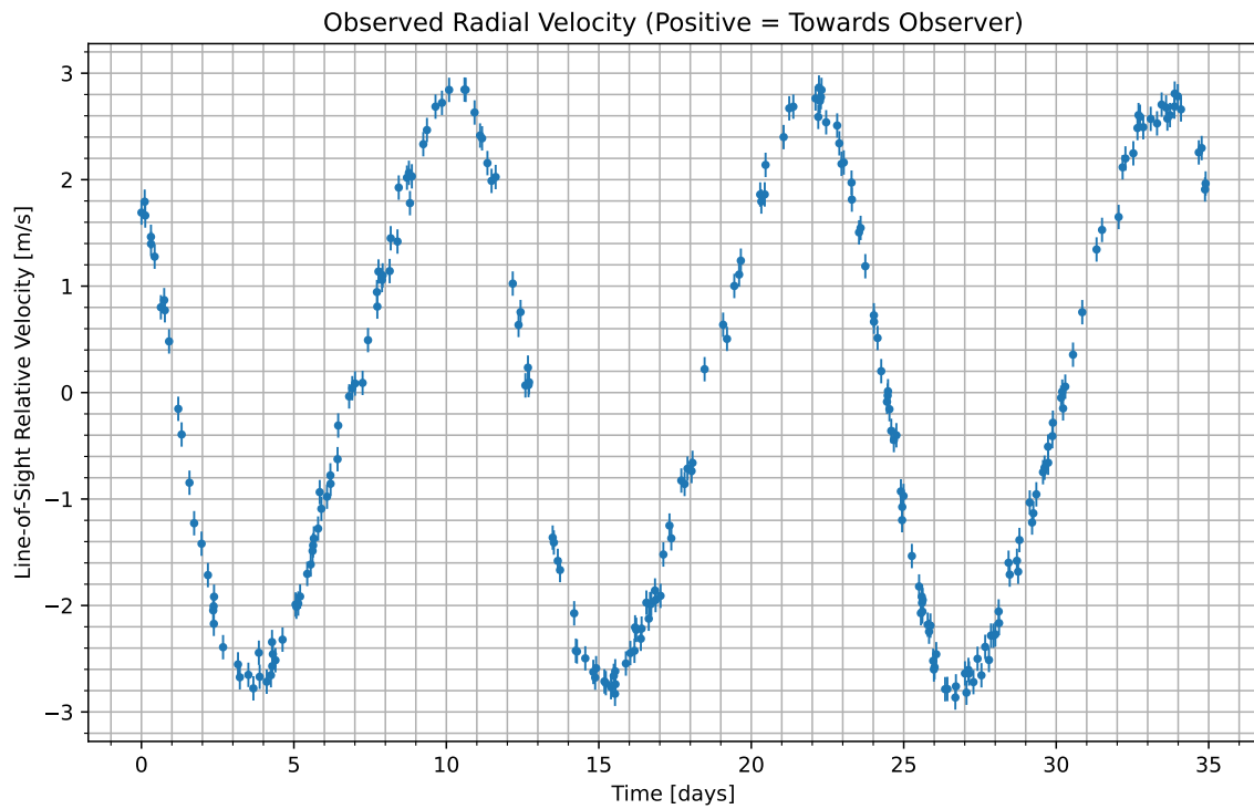
Figure 1: We have isolated the radial velocity of the host star due to the candidate planet. Data begins at UTC 2072-05-23/06:38. Positive values indicate the velocity at which the star is moving towards us; negative indicate the velocity at which it is moving away.
